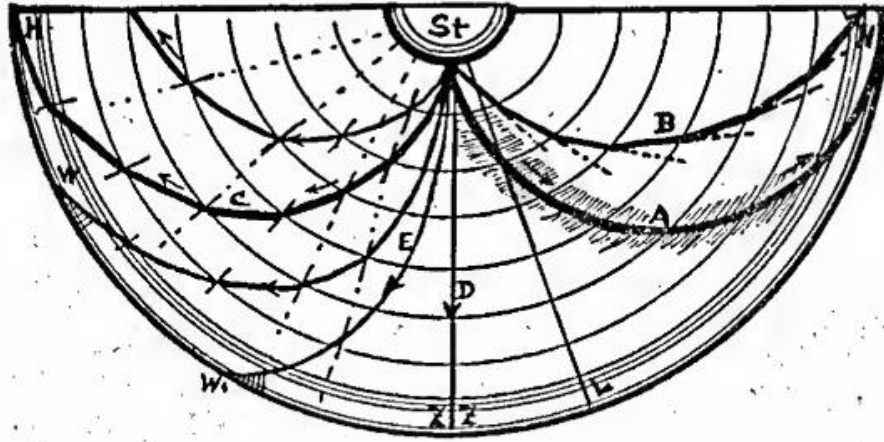
Light bending in space in curves. Circumference earth ball, the sun at St above. St. Star ball. The fine circles are layers and densities, billionfold to think. Strokes = refraction away from the perpendicular.
