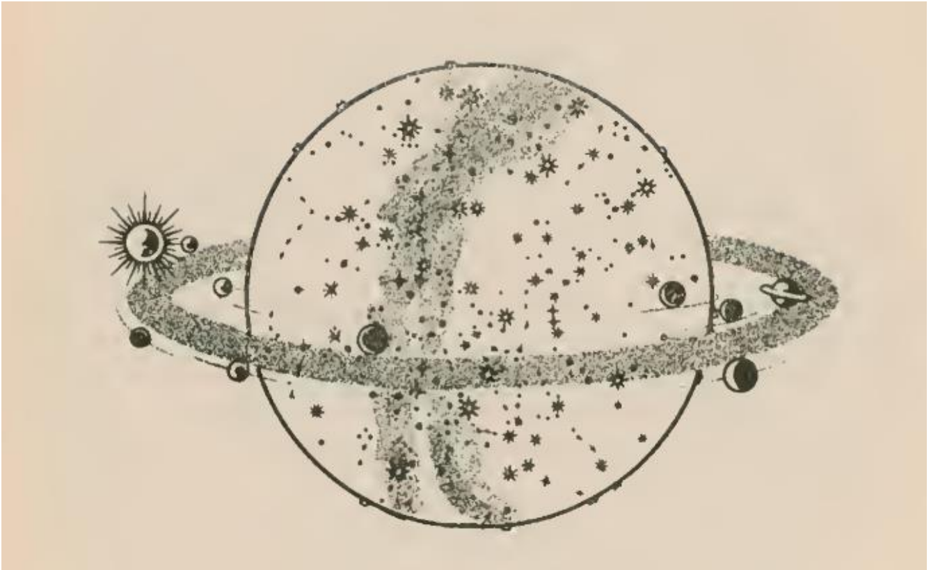
The arrangement of the stars in the Geocosmic sky
