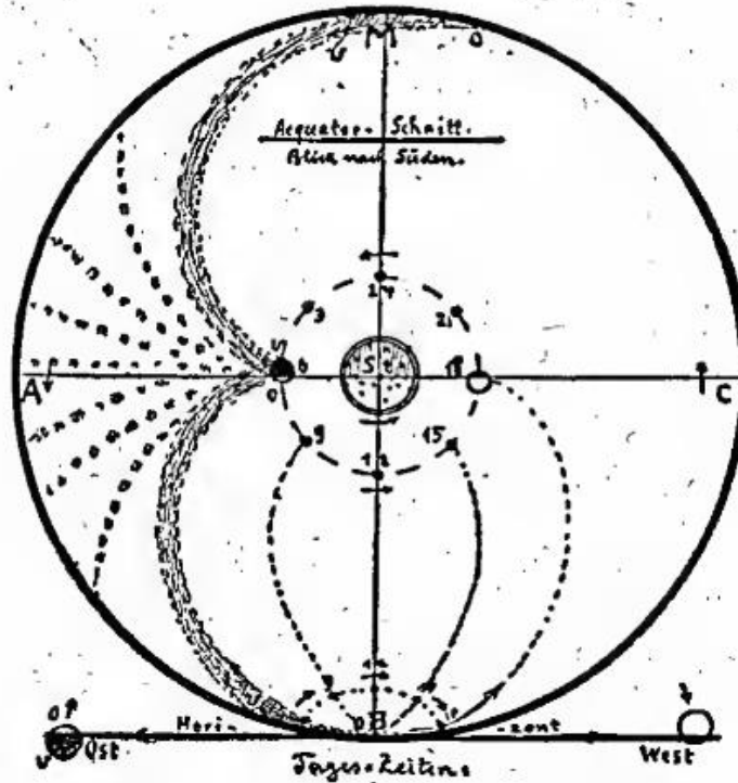
Sun course in the day around the earth.
